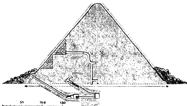
SECTION OF THE THIRD PYRAMID, SHOWING PASSAGES.
