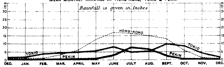
MEAN MONTHLY RAINFALL AT HONG-KONG, TOKIO &amp; PEKIN
