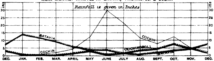
MEAN MONTHLY RAINFALL AT BATAVIA, TRICHINOPOLI &amp; COCHIN
