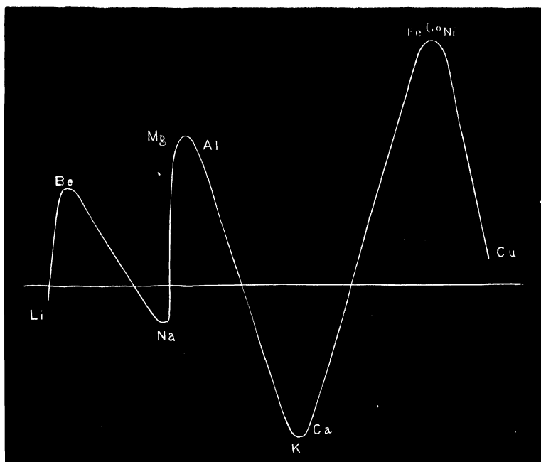
FIG. 1.—Periodicity of Electric Touch . Abscissa represents the atomic weight; ordinate the electric touch positive or negative.
