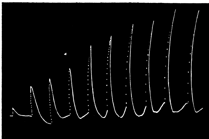
FIG. 8.—The ' staircase ' enhancement of response in plant.
